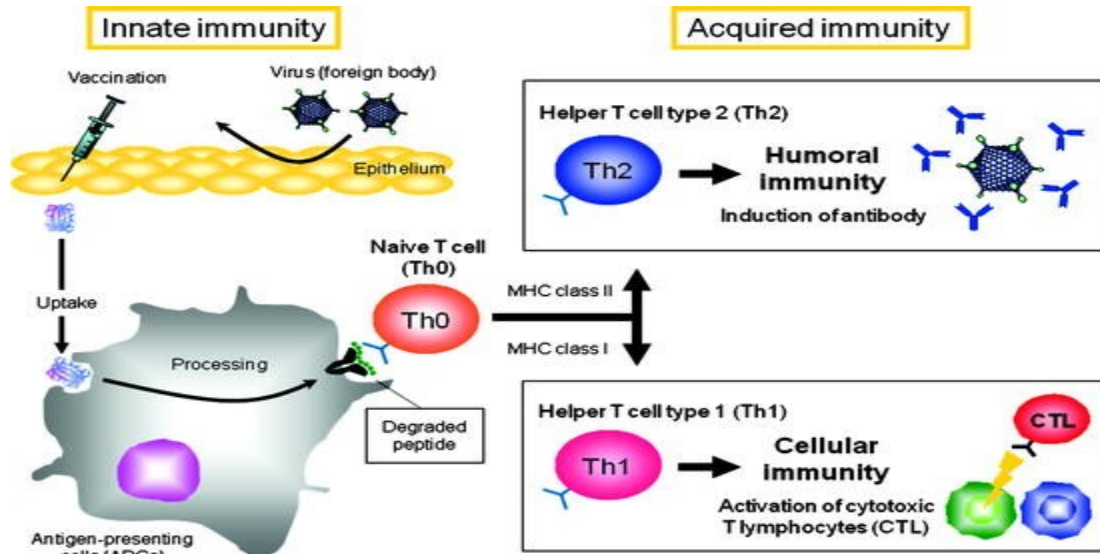
Schematic showing pathways for Th1 and Th2 acquired immunity (a.k.a. adaptive immunity), and roles of MHC class I and class II. Figure from Akagi, Baba and Akashi 38 .
